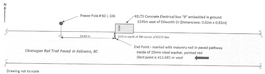
DETAIL B - END POINT (Plan View)
